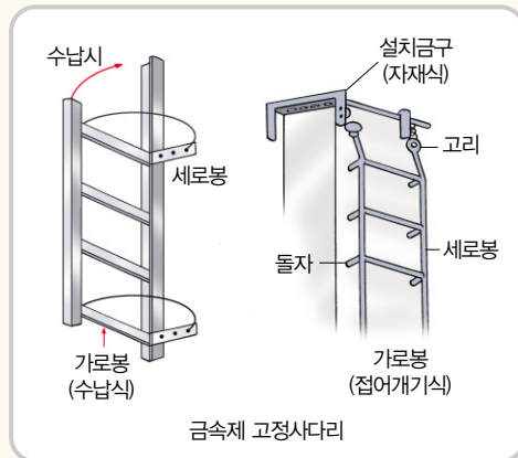
[피난사다리]
