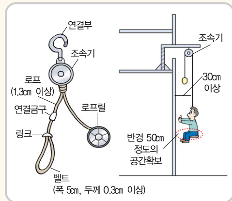
[완강기]
